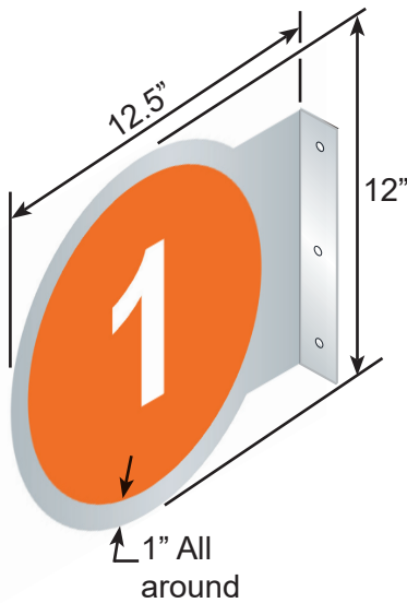
(Above) SGN FLAG 1.5X12X12.5 (WITHOUT DECALS) Part No. 764197
