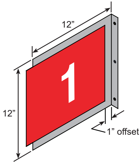
SGN FLAG 1.5X12X13 HIGHWIND (WITHOUT DECALS) Part No. 764417
