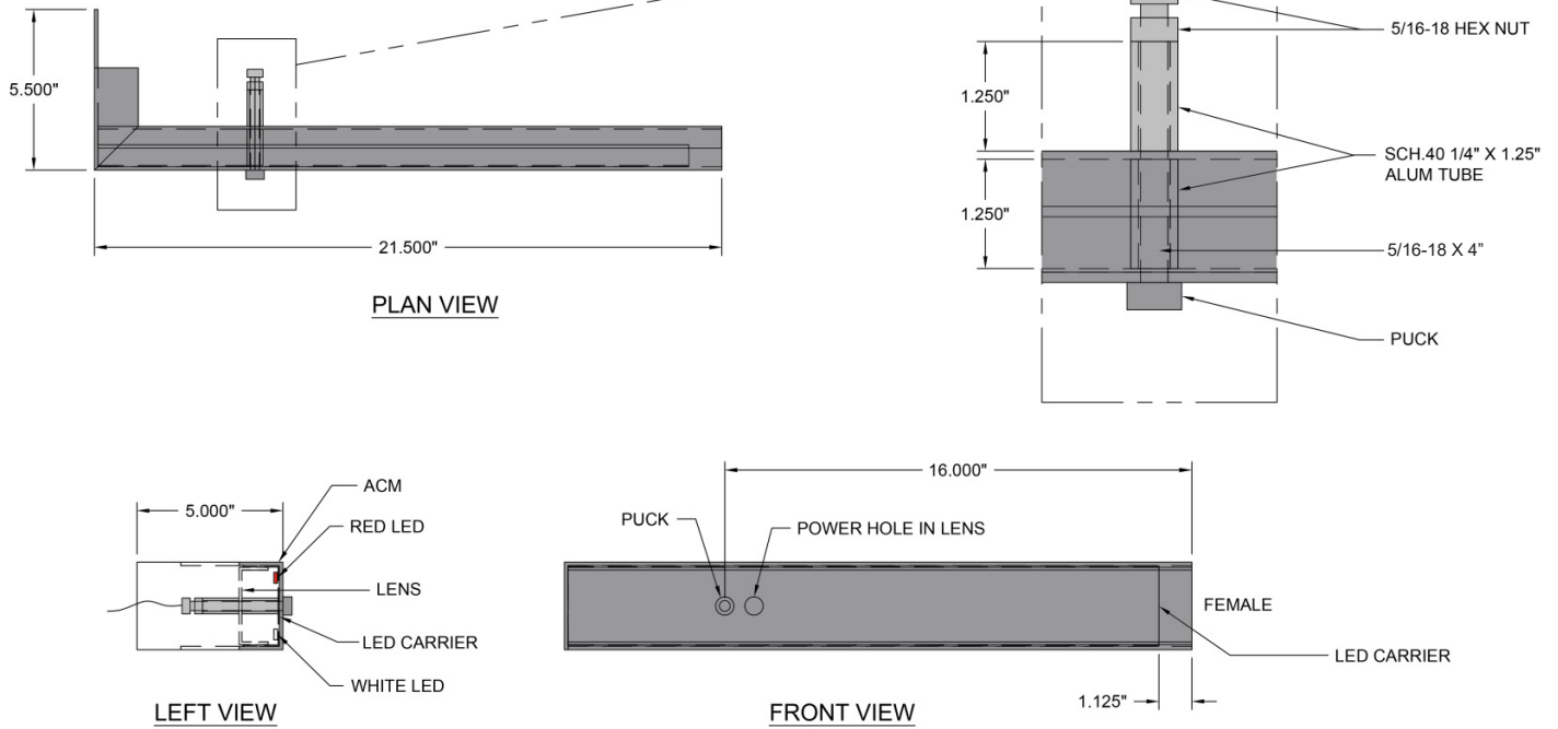
End Cap Rail Female - DWG. 8
