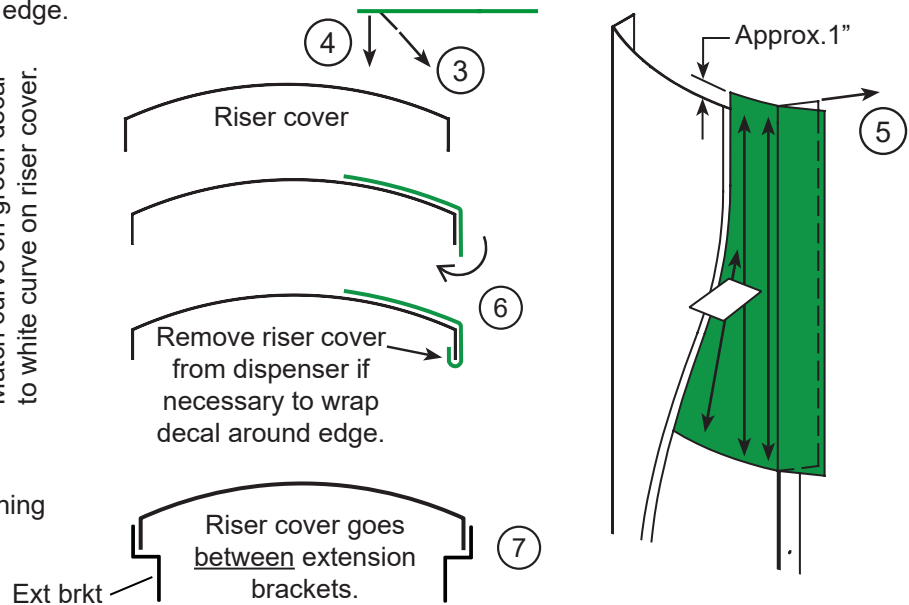
DECAL RISER COVER 44.00X17.04 66RF, P76 WAVE DSL, PN 767665, ENCORE, ENCORE S, ADVANTAGE
