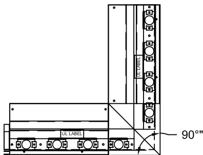
STANDARD CORNER
