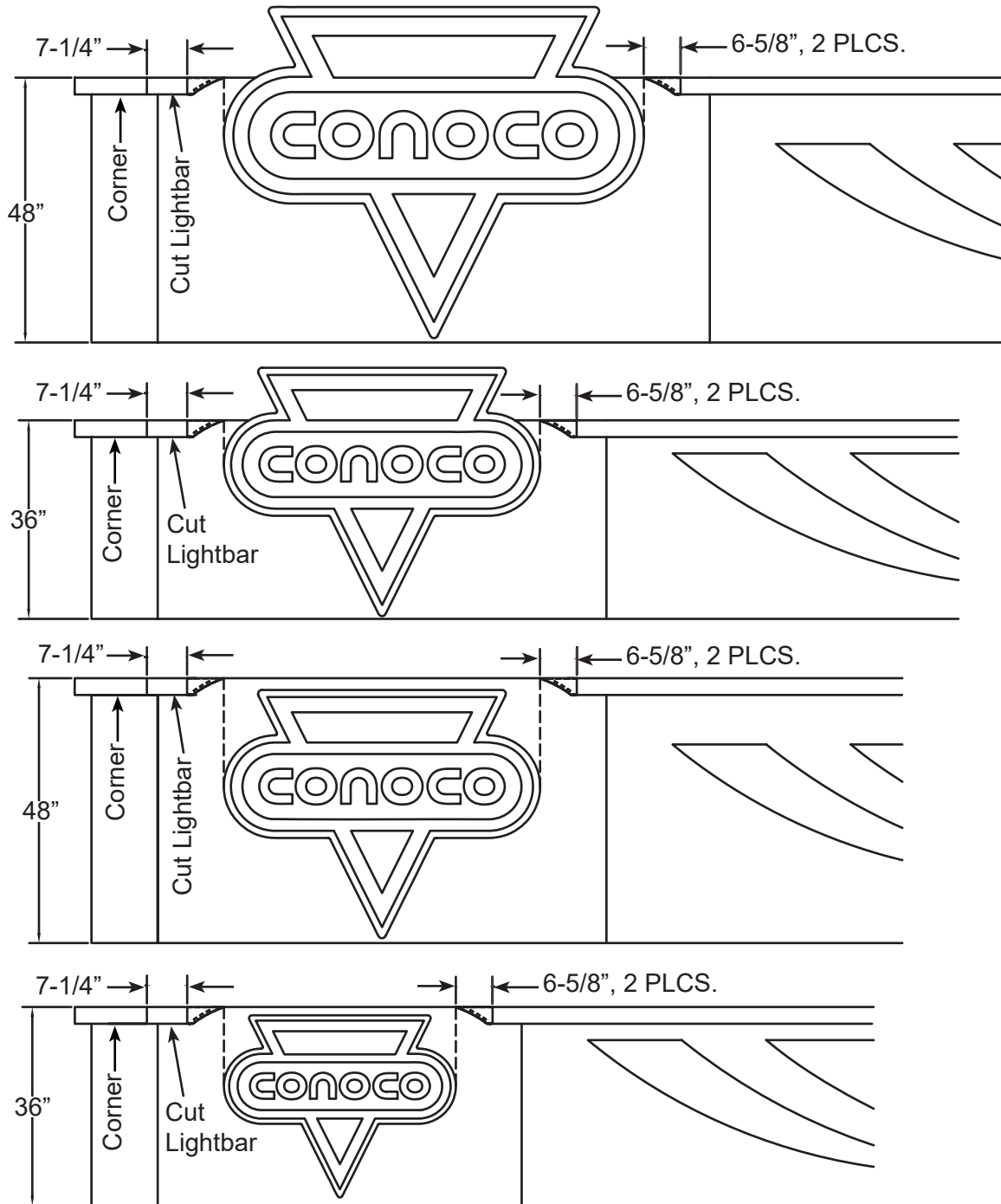
FIGURE B PLACEMENT OF RADIUS CAPS AROUND LOGOS
