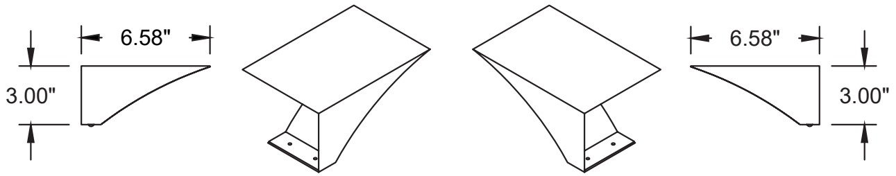
End Cap Set LH & RH Curves Logo for Downlighter Part Number 644790 (Silver)
