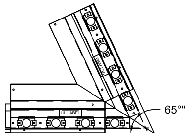
ACUTE CORNER
