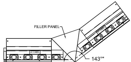
OBTUSE CORNER
